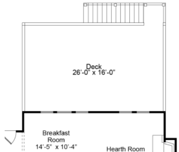
OPTIONAL DECK/COVERED PATIO
