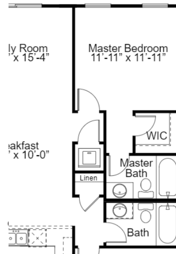
OPTIONAL FIRST FLOOR LAUNDRY
