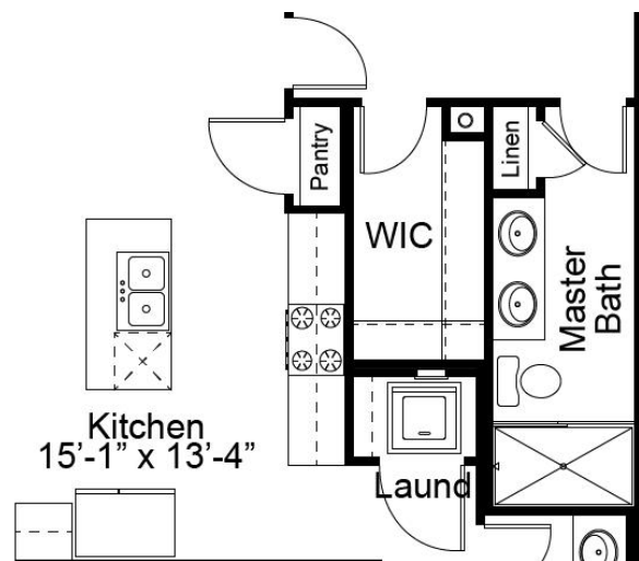
OPTIONAL FIRST FLOOR LAUNDRY
