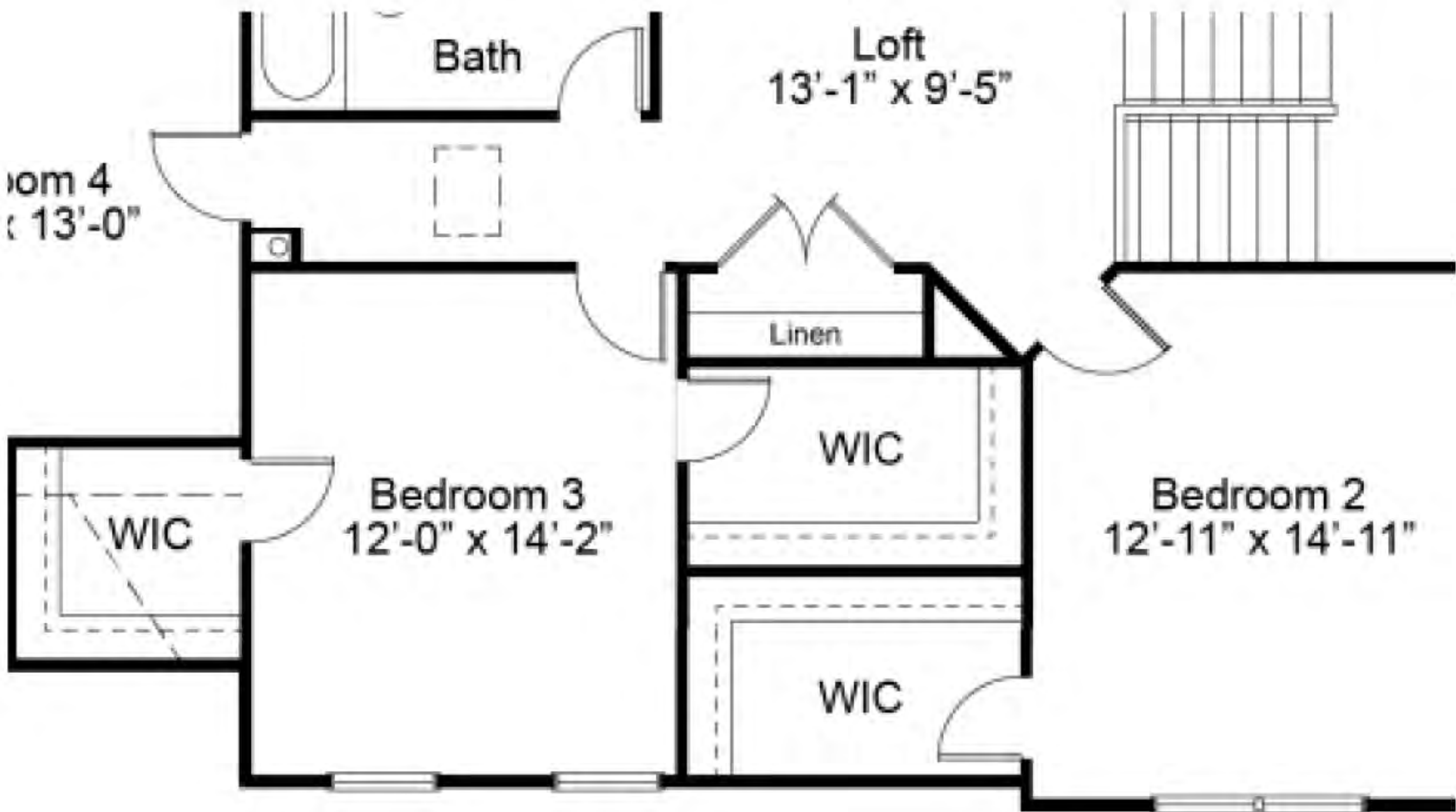
SECOND FLOOR WITH FIRST FLOOR LAUNDRY
