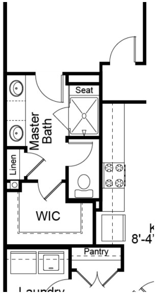
OPTIONAL SPA MASTER BATH
