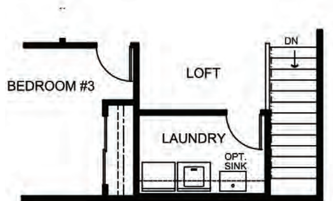
OPTIONAL SECOND FLOOR LAUNDRY
