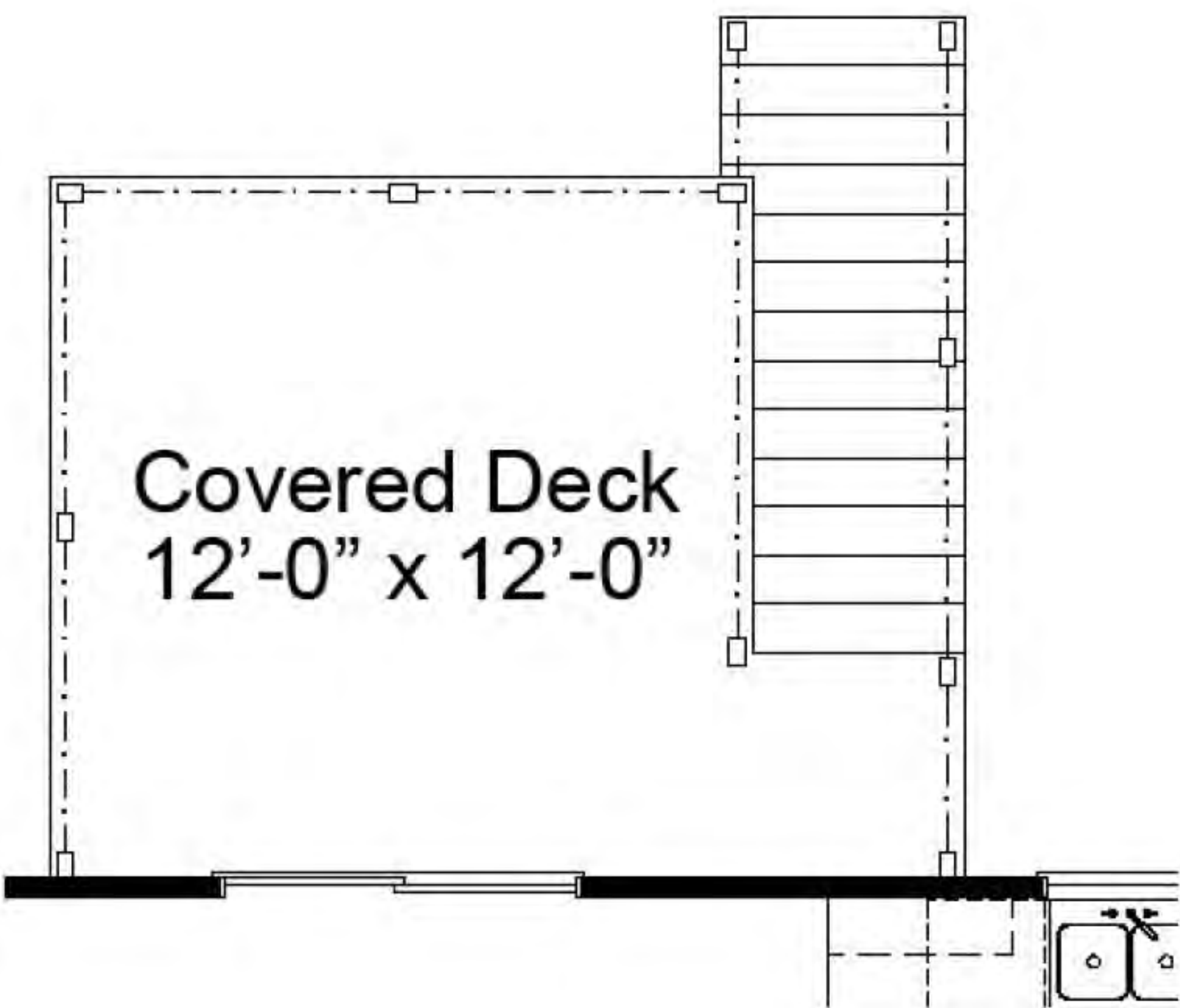
OPTIONAL DECK/COVERED PATIO
