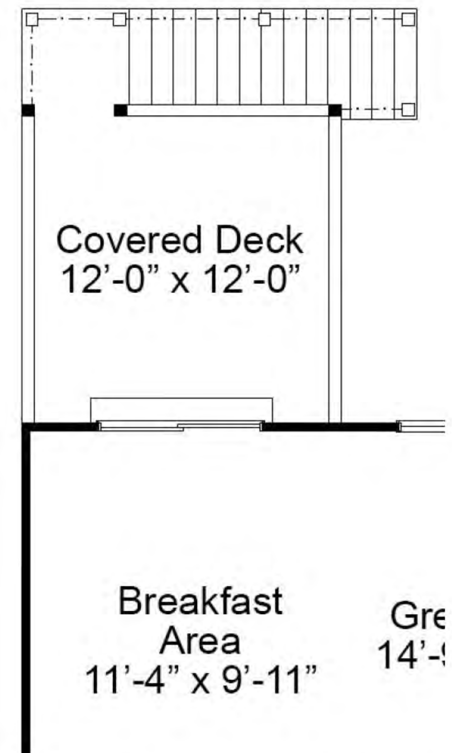
OPTIONAL DECK/ COVERED PATIO
