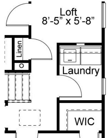
OPTIONAL SECOND FLOOR LAUNDRY
